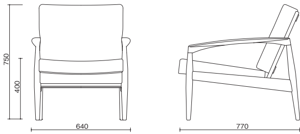
size W640×D770×H750 (SH400) mm
